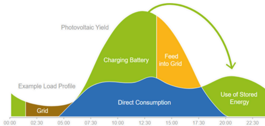
Figure 1: Generic storage arbitrage with solar integration
